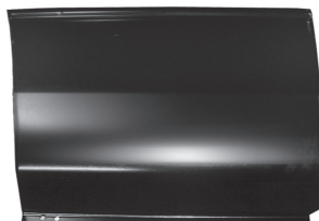
BED: LWR FRT SECT (Left) ..... 1582-141L BED: LWR FRT SECT (Right) ..... 1582-142R 21.75"W x 15.5"H, 6.5' Bed
