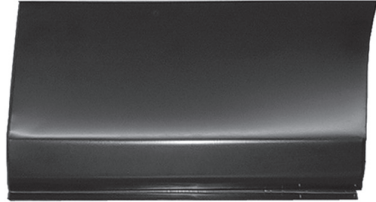
QTRP: LWR FRT SECT (Left) ..... 0871-241L QTRP: LWR FRT SECT (Right) ..... 0871-242R 20"W x 13"H, Blazer 2 Door
