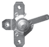
DR: SHORT RELAY LATCH (Left) .... 0849-811L DR: SHORT RELAY LATCH (Right) . 0849-812R (67-71)
