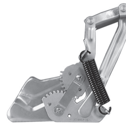
HOOD: HINGE (Left) ..... 0847-041L HOOD: HINGE (Right) ..... 0847-042R (55-57) Spring Included
